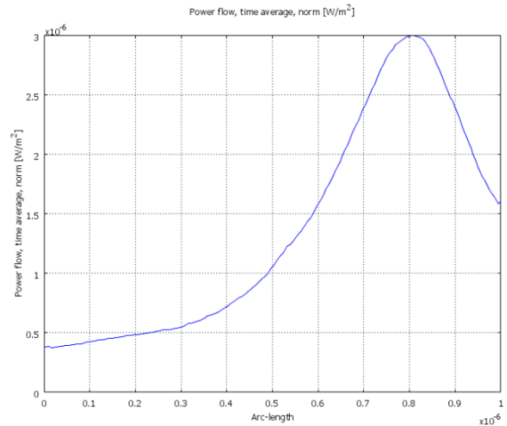
Fig. 8. Normalized output power for (0.15a).
