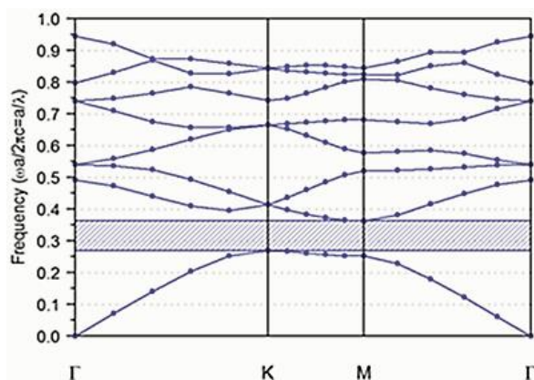
Fig. 2. Band diagram for TM polarization in a triangular lattice of AlGaAs rods.
