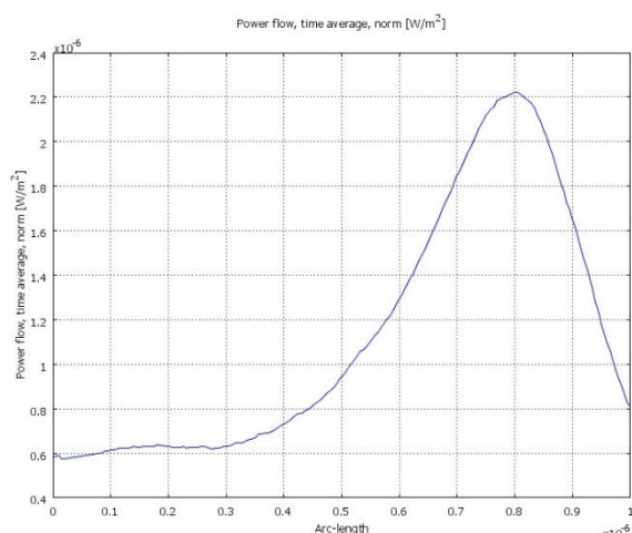
Fig. 9. Normalized output power for (0.16a)
