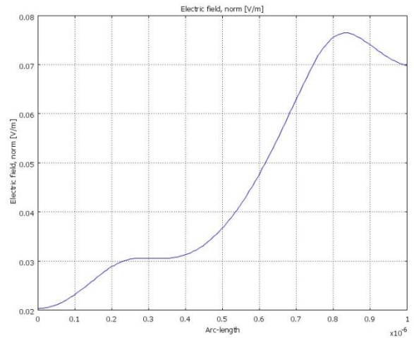
Fig. 7. Normalized component electric field for (0.16a).
