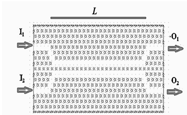
Fig. 1. A directional coupler switch based on Photonic crystal.
