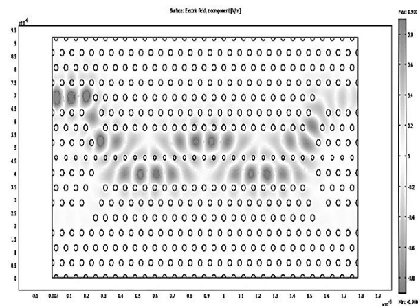
Fig. 4. All-optical switch in linear state.
