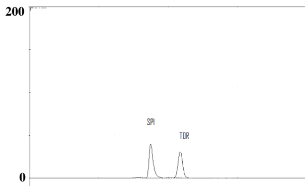
Fig. 1. Isocratic RP-HPLC chromatogram of TOR and SPI with detection at 252 nm.
