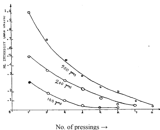
Fig. 1. (k) ML intensity of camphor crystal with repeated crushing using impulsive devices.
