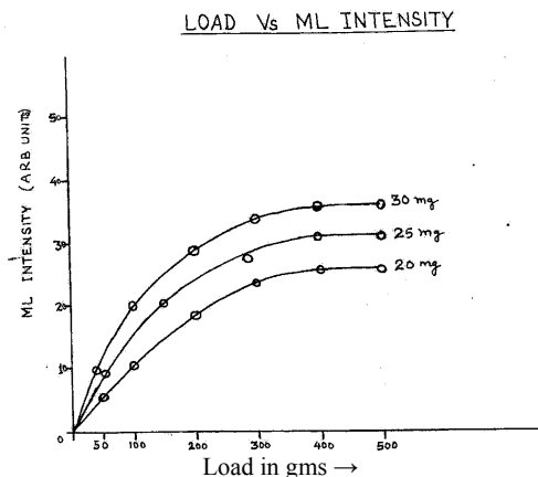
Fig. 1. (g) ML intensity of camphor crystal at constant Mass using impulsive device.
