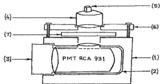
Fig. 1. (b) Photomultiplier tube housing with band pass filter for spectral studies: (1) Wooden block (2) Metal cylinder (3) P. M. Tube (4) Lucite Plate (5) Crystal (6) Metal Platform (7) space for keeping band pass filter.
