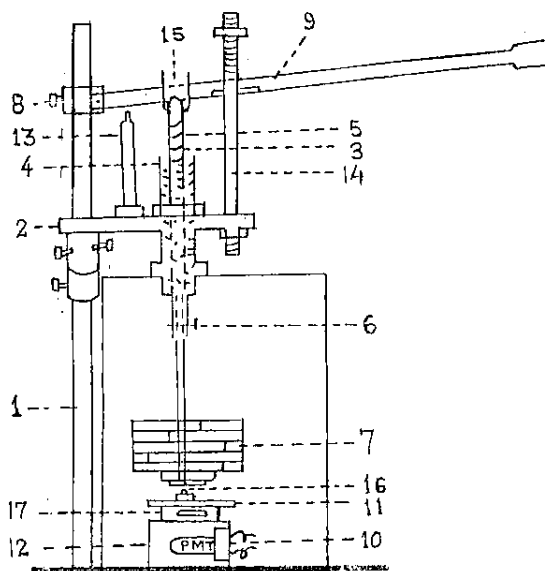
Fig. 1. (a) A schematic diagram of the device used for the determination of mechanoluminescence by static method (1) Vertical stand (2) Platform (3) Cylinder with uniform bore just fitting cylinder spring (5) Exactly fitting solid rod passing through the central hole of the platform (6) Hook for supporting hanger, (7) load and adjustable hanger, (8) clamp for lever, (9) lever rod (10) mount of the PM tube (11) glass plate for mounting the crystal (12) P.M. tube IP28 (13) adjustable rod (14) guiding rod for lever (15) guide for central rod (16) crystal (17) filter.
