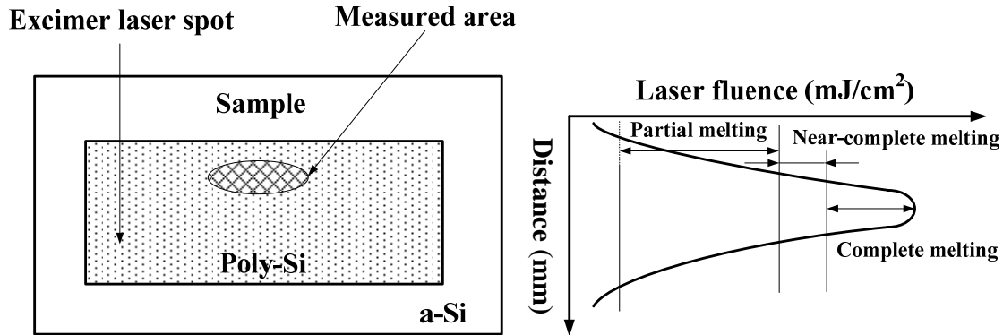
Fig. 4. Schematic illustration of the measured area.
