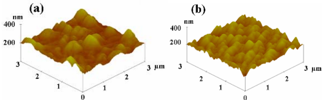
Fig. 5. Surface topography measured by AFM of poly-Si films in the SLG regime for (a) frontside ELC (RMS roughness= 21.192 \text{ nm} ) and (b) backside ELC (RMS roughness= 16.263 \text{ nm} ). Excimer laser energy density for frontside ELC and backside ELC is 190 \text{ mJ/cm}^2 and 175 \text{ mJ/cm}^2 , respectively.
