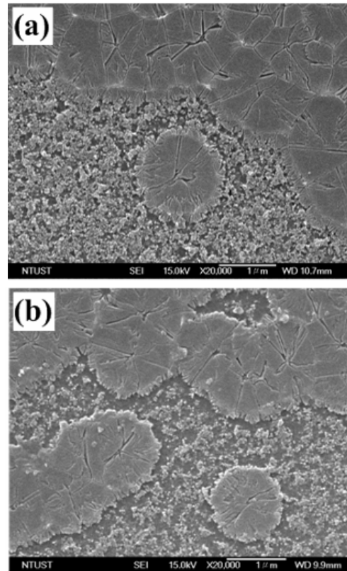
Fig. 8. SEM micrographs of complete melting of Si thin films for (a) frontside and (b) backside ELC. Excimer laser energy density for frontside ELC and backside ELC is 210 \text{ mJ/cm}^2 and 195 \text{ mJ/cm}^2 , respectively.
