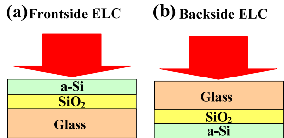
Fig. 1. Schematic illustration of (a) frontside ELC and (b) backside ELC.
