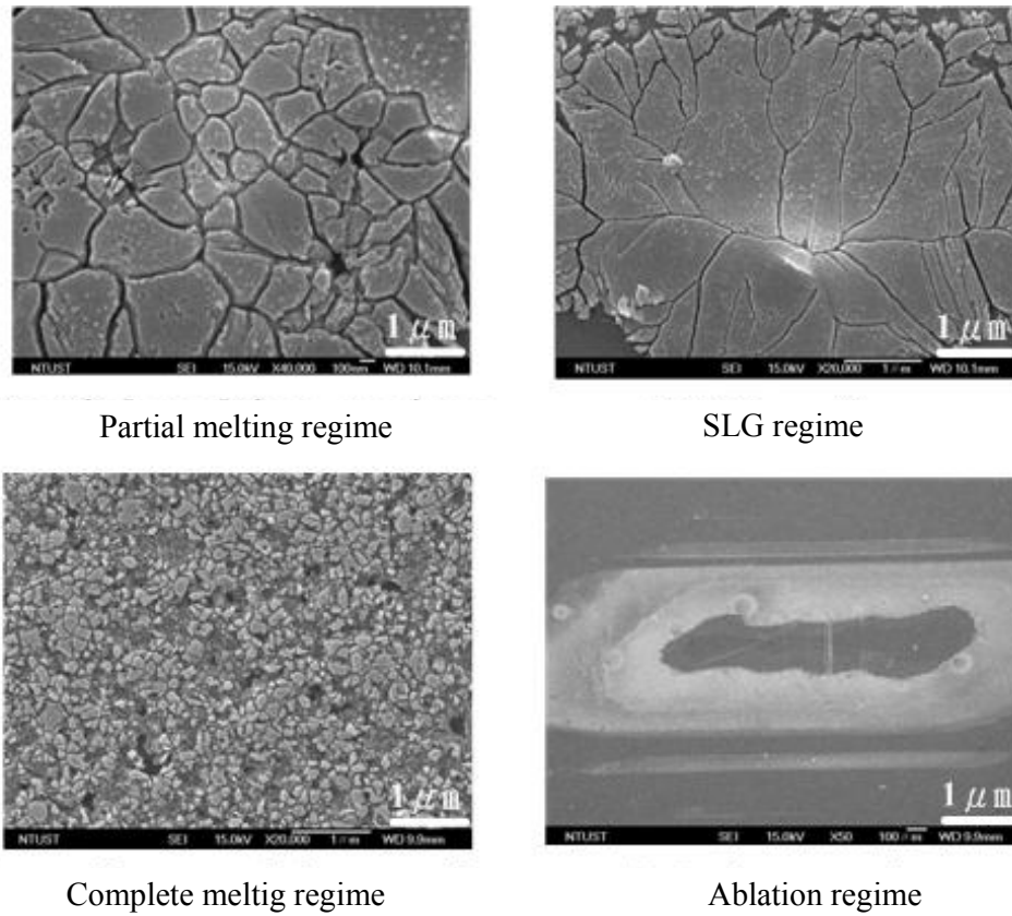
Fig. 2. FE-SEM images of Secco-etched poly-Si films in four distinct regrowth regimes. Excimer laser energy density for the partial melting regime, SLG regime, complete melting regime, and ablation regime is 130 \text{ mJ/cm}^2 , 190 \text{ mJ/cm}^2 , 210 \text{ mJ/cm}^2 , and 230 \text{ mJ/cm}^2 , respectively.
